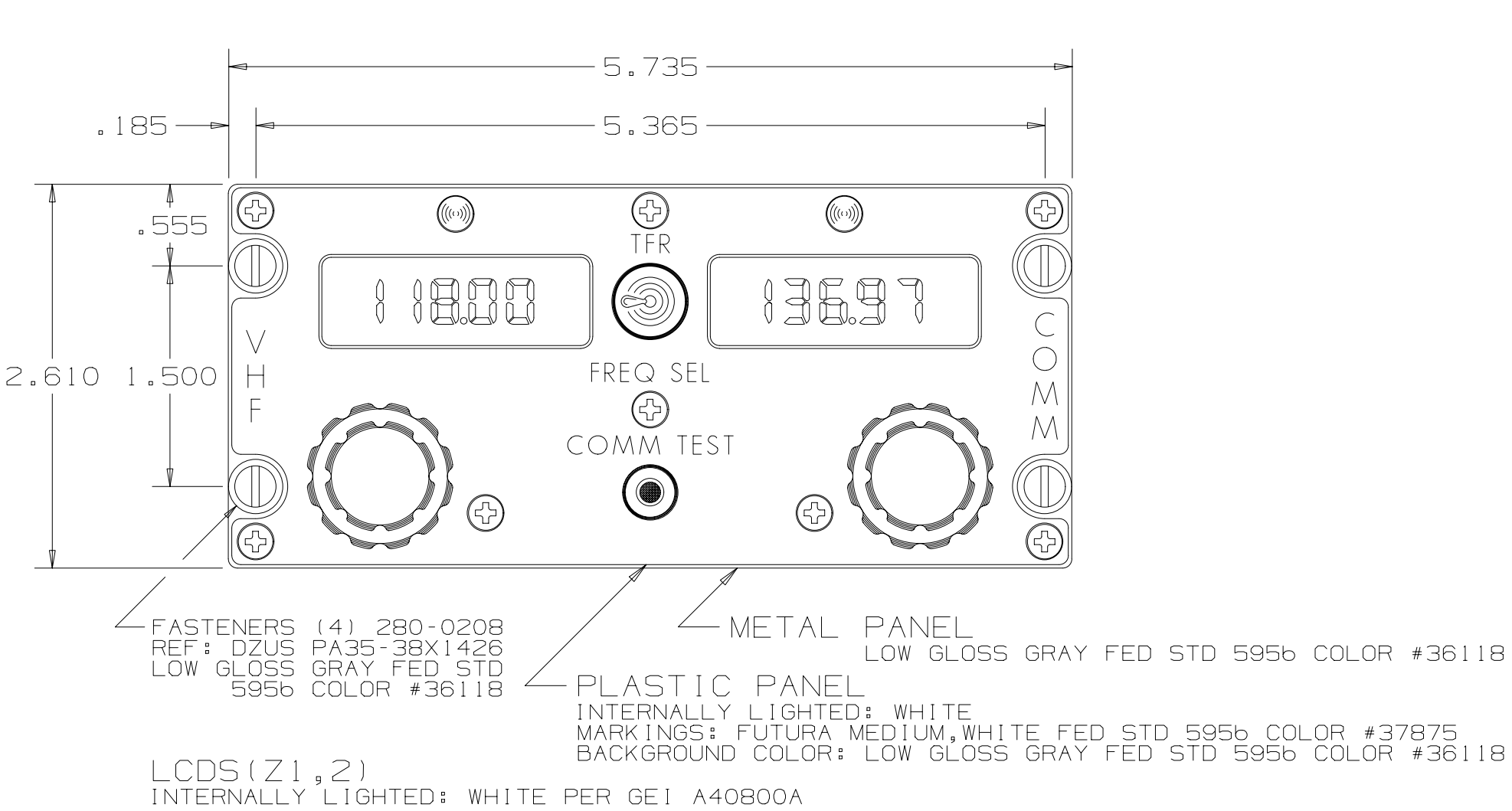
FRONT VIEW FULL SCALE
